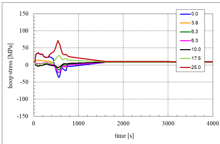
Figure 4-4. ADS transient => Core shroud wall hoop stress time history (0 is at inner surface).
