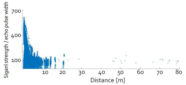
Figure 15. Light fog (visibility 40 m) measurements for the Ibeo 905 nm LiDAR
