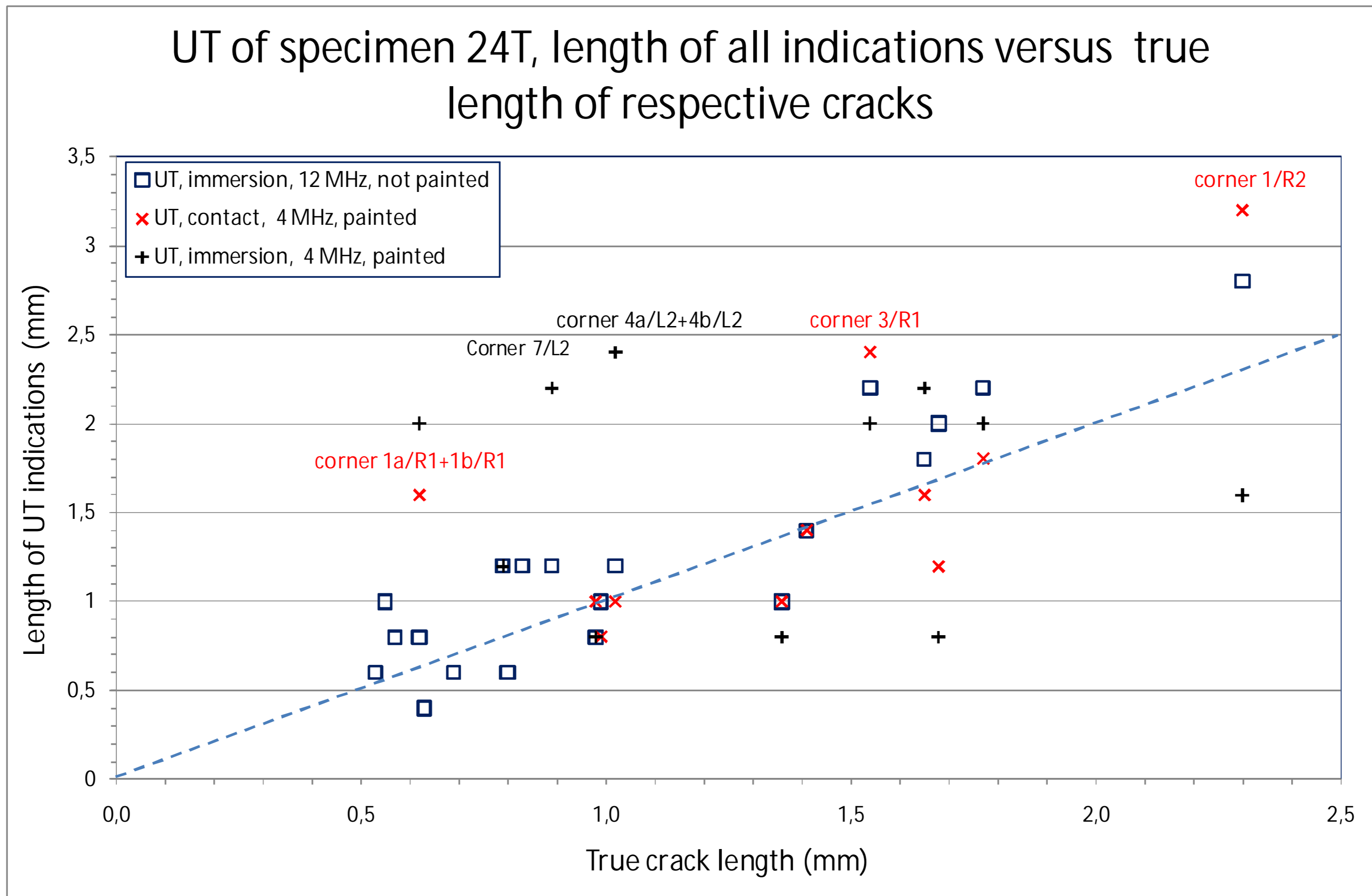
Figure 22: The specimen 24T, the UT length of all detected fatigue crack indications versus true length of cracks. 12 MHz immersion technique was applied before painting and 4 MHz contact and immersion technique were applied after painting. Picture by courtesy of VTT.
