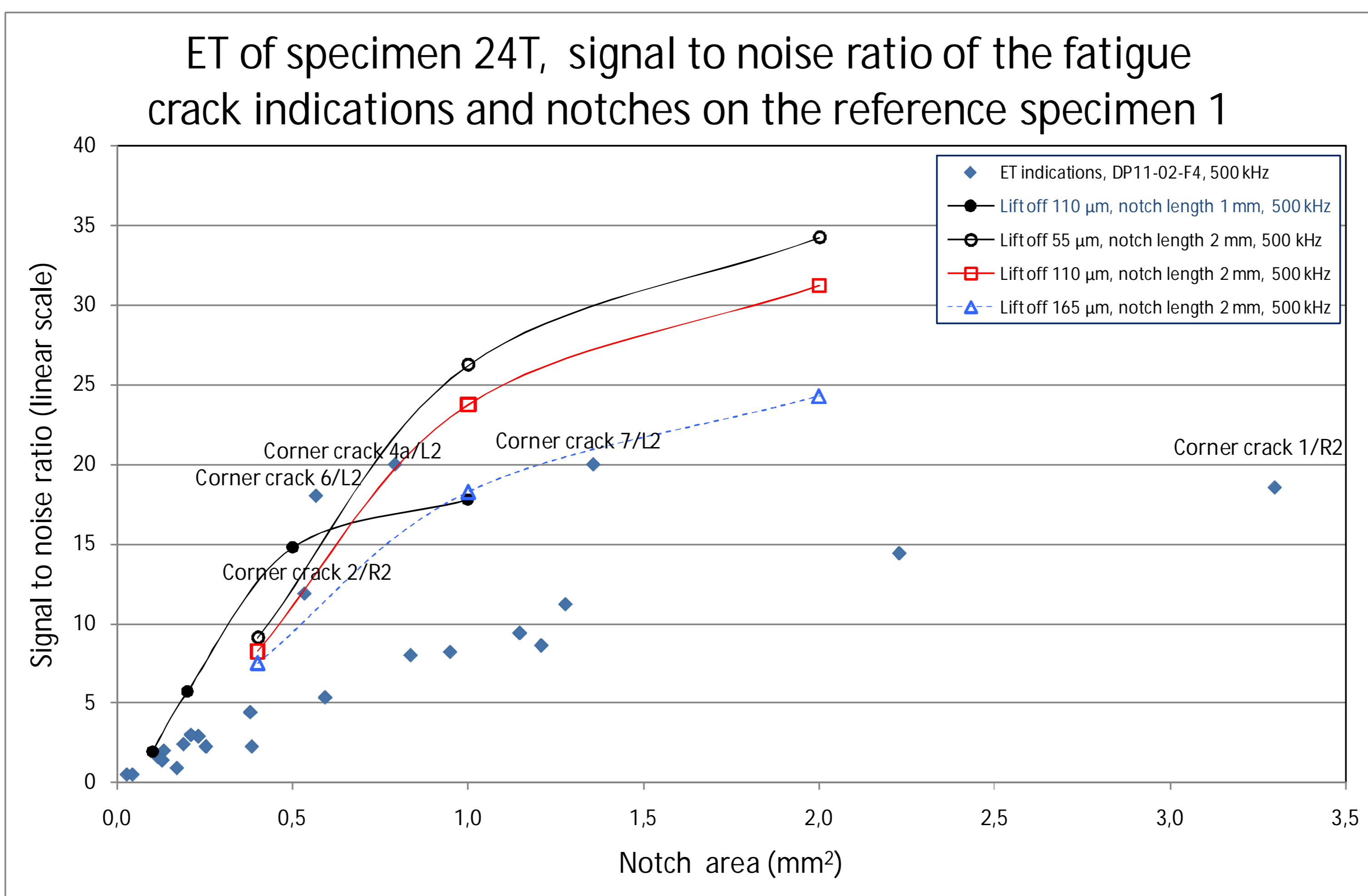
Figure 23: The signal to noise ratio of all fatigue crack indications detected from the R and L sides of the specimen 24T (blue dots \blacklozenge ). The four calibration curves were created using reference notches on planar area and different lift-off values (distance between the transducer and the surface). The transducer DP11-02-F4 was used. The applied ET frequency was 500 kHz. Picture by courtesy of VTT.
