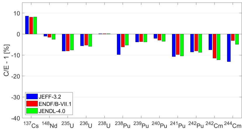
Figure 4. Calculated/Measured - 1 isotopic concentrations in % when normalizing to sample burnup from 148 Nd measurement.
