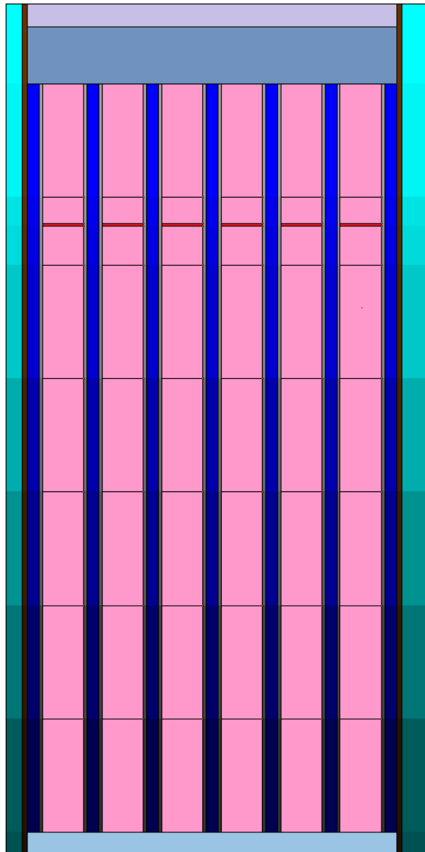
Figure 3. Three dimensional Serpent model of the Gundremmingen-A assembly B23 in xz-plane. The pink pillars represent the fuel and the red thin discs between the pink pillars picture the axial level of sample I2680.
