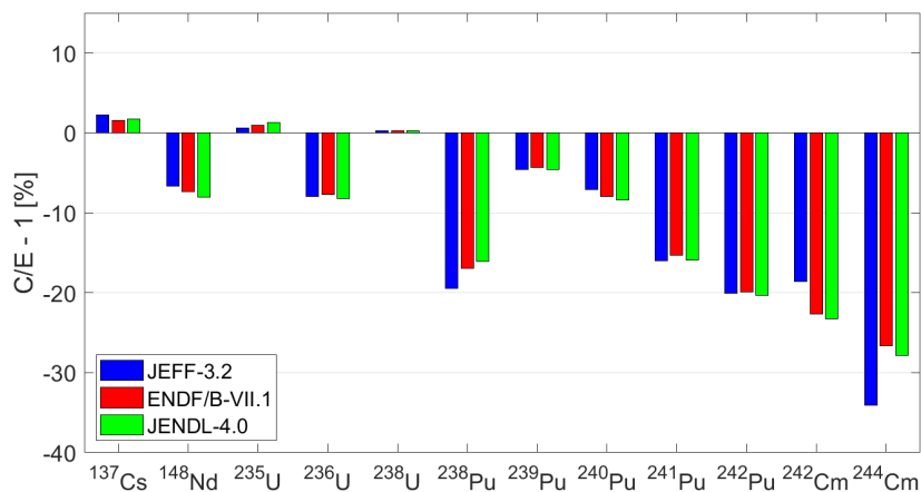
Figure 6. Calculated/Measured - 1 isotopic concentrations in % when normalizing to measured assembly burnup.
