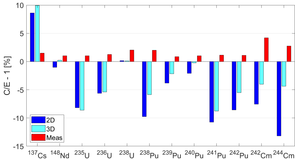
Figure 9. Calculated/Measured - 1 isotopic concentrations in % in the 2D and 3D calculations using ^{148}\text{Nd} measured burnup and JEFF-3.2 cross sections. Measurement uncertainties from SFCOMPO-2.0 are presented in red bars.
