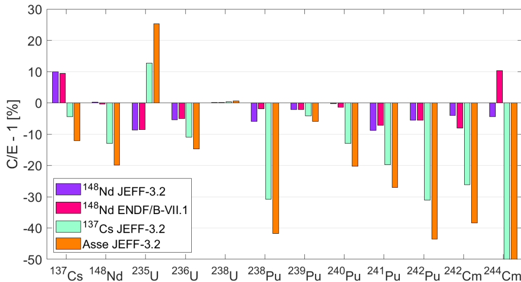
Figure 8. Calculated/Measured - 1 isotopic concentrations in % in the 3D calculations.
