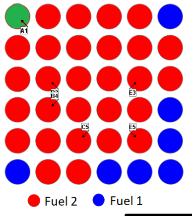
Figure 1. Modelled assembly B23 [2]. The calculated sample is presented in green colour.
