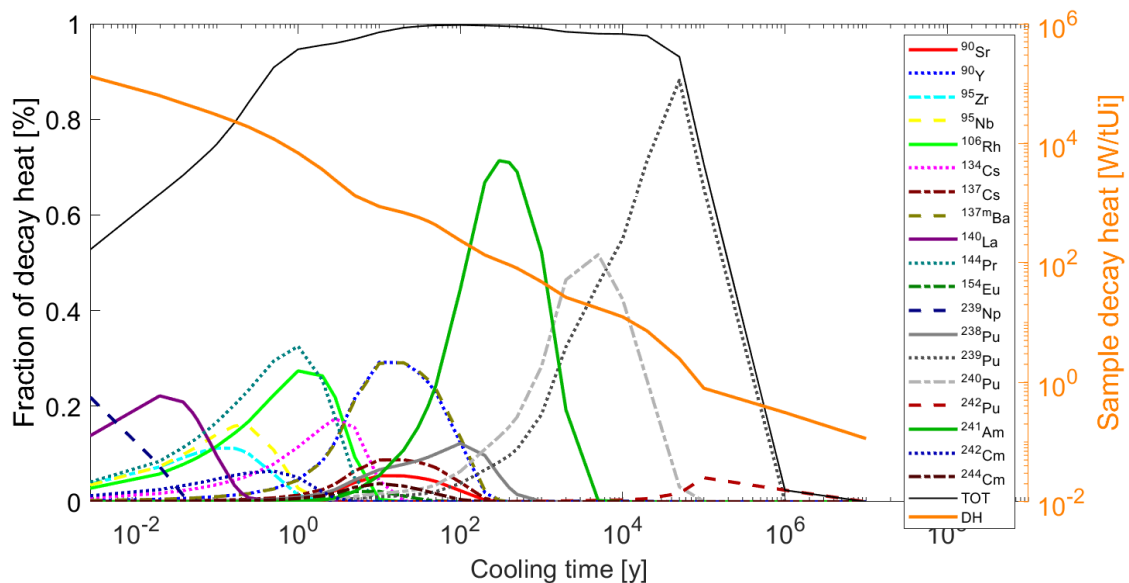
Figure 7. Contribution to sample 12680 decay heat by the most significant decay heat producing nuclides. TOT stands for the total fraction of decay heat from all the nuclides presented in the figure.
