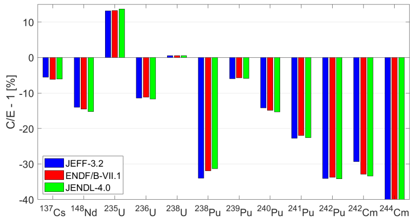
Figure 5. Calculated/Measured - 1 isotopic concentrations in % when normalizing to sample burnup from 137 Cs (DA) measurement.
