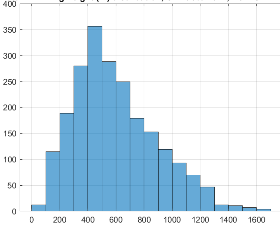
Autumn mixing height (m) distribution, Oikiluoto 2012, from SILAM data
