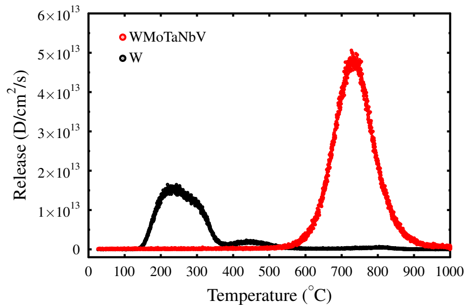
Figure 2. Thermal release D signals from WMoTaNbV and W with 10 °C/min heating rate.
